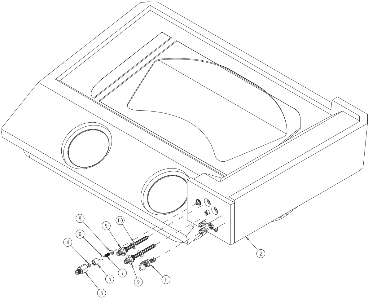
Figure 9. Carbonator Tank Assembly
