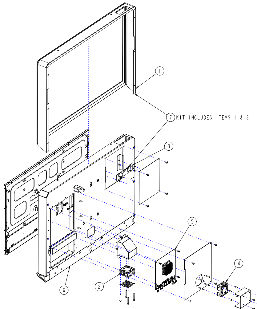
Figure 11. Door Assembly
