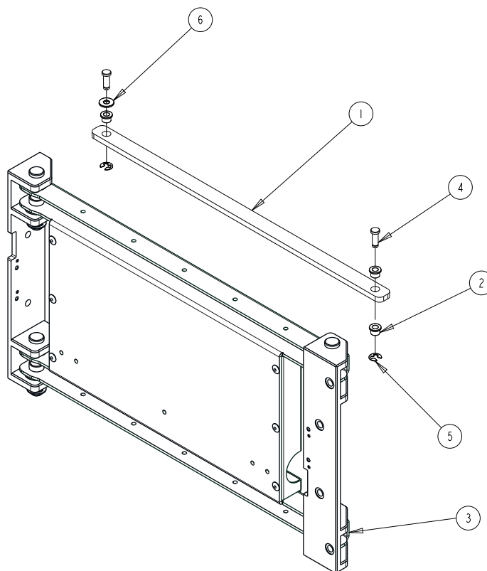
Figure 2. Hinge Assembly
