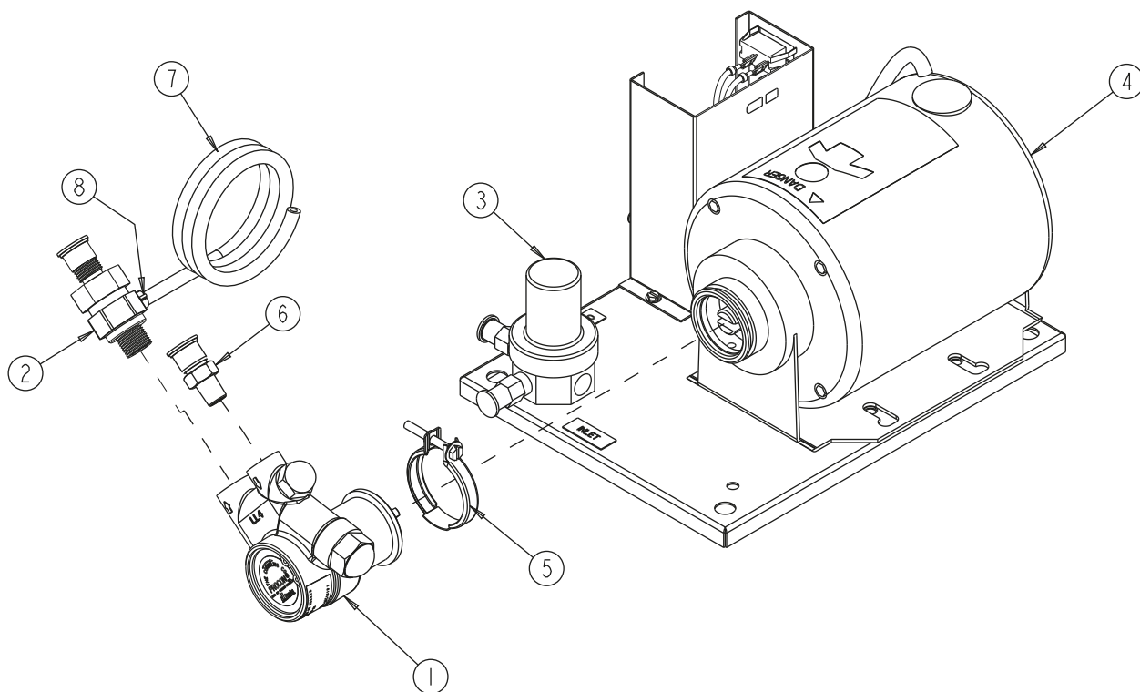
Figure 10. Pump and Motor Assembly
