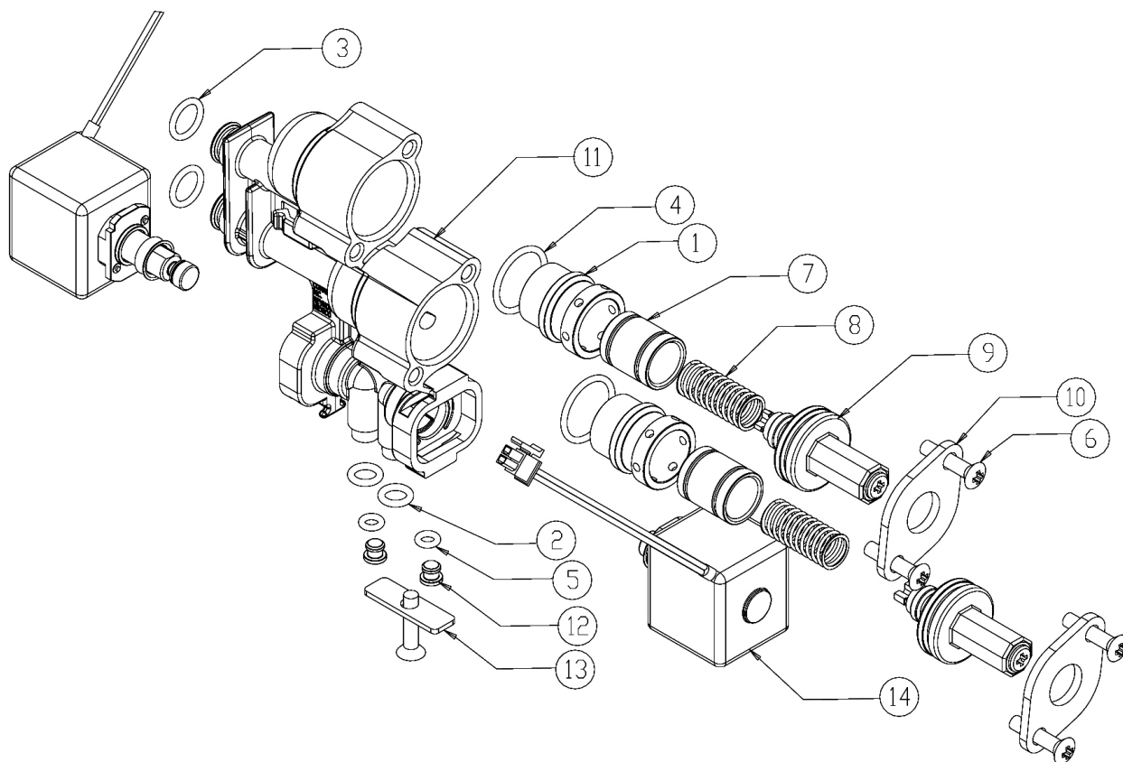
Figure 13. Valve Assembly
