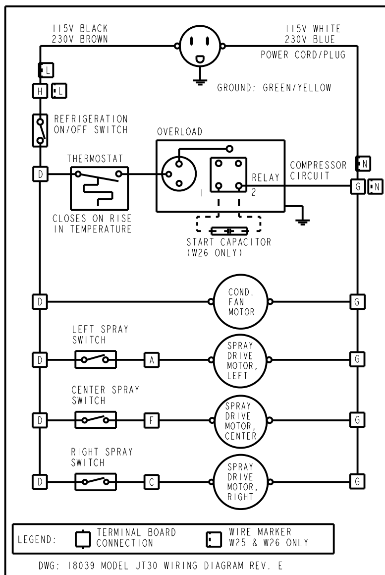
Figure 11. JT30 Wiring Diagram
