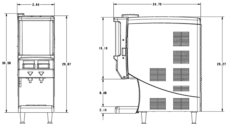
Figure 1. Unit Dimensions
