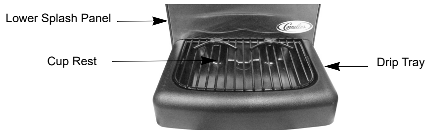
Figure 12. Drip Tray and Cup Rest
