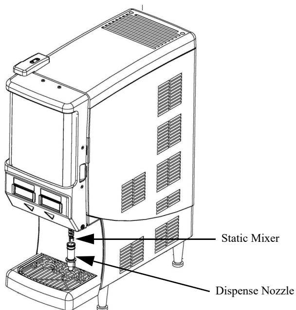
Figure 9. Dispense Nozzle
