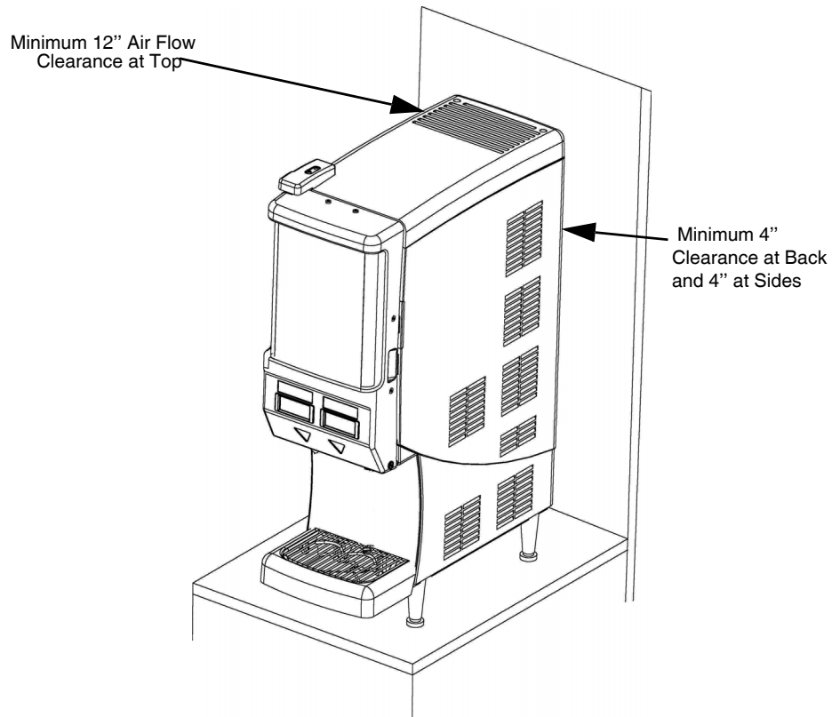
Figure 5. Minimum Clearances
