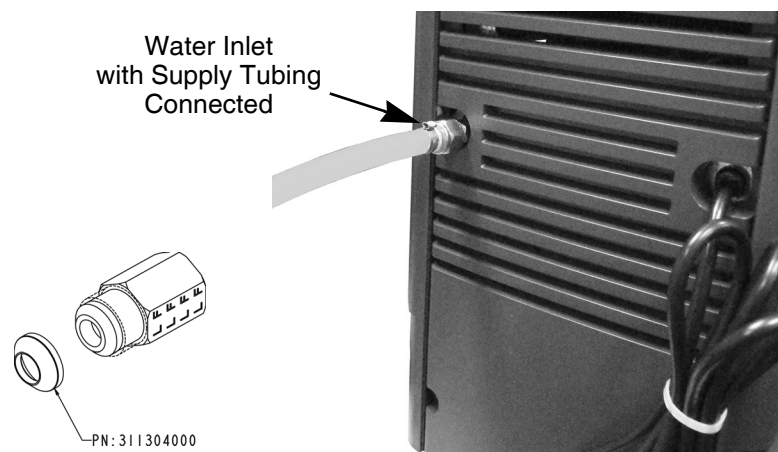
Figure 8. Water Supply Connection on Rear of Unit
