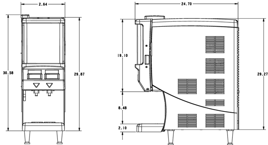
Figure 1. Unit Dimensions
