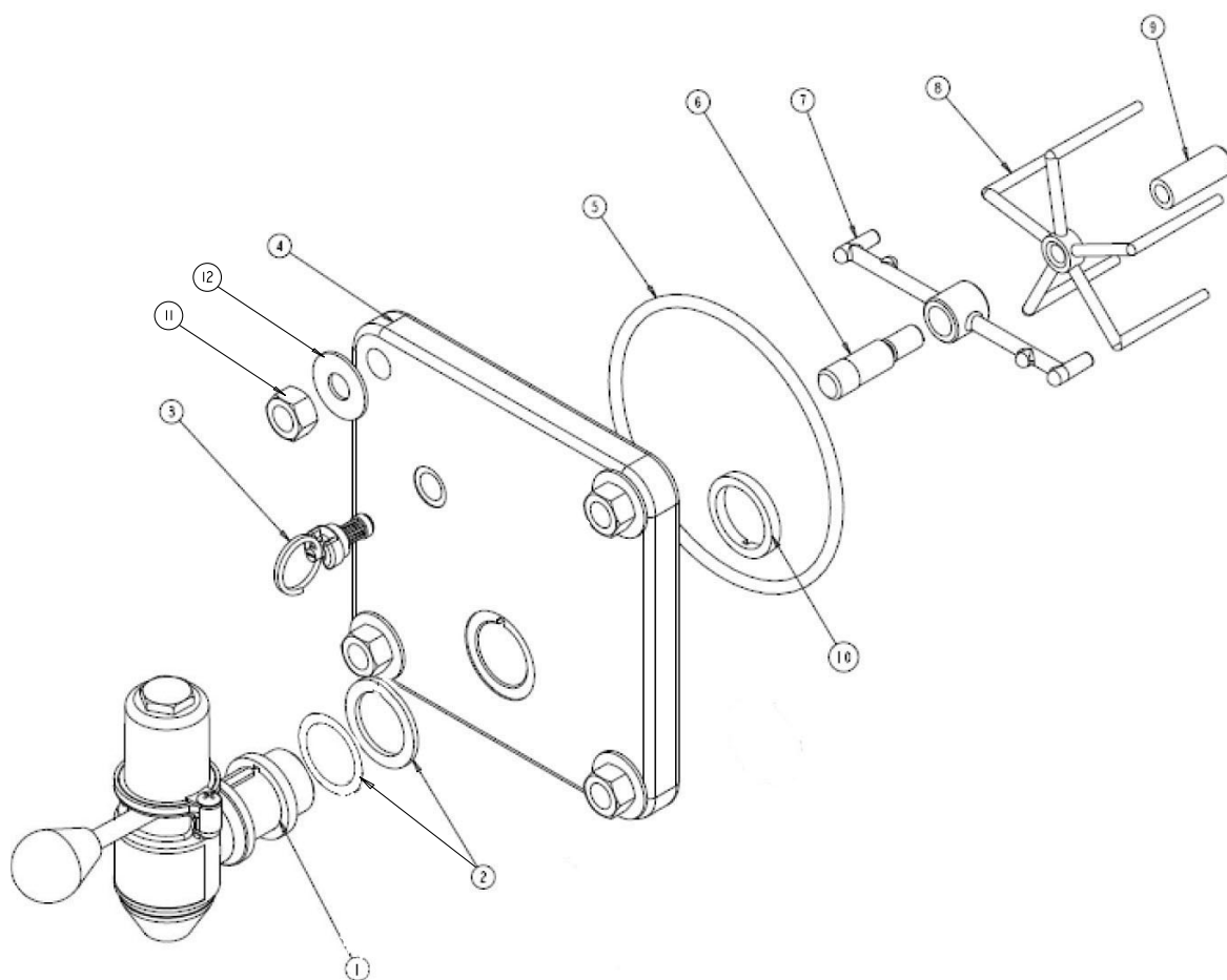
Figure 3. Faceplate Assembly
