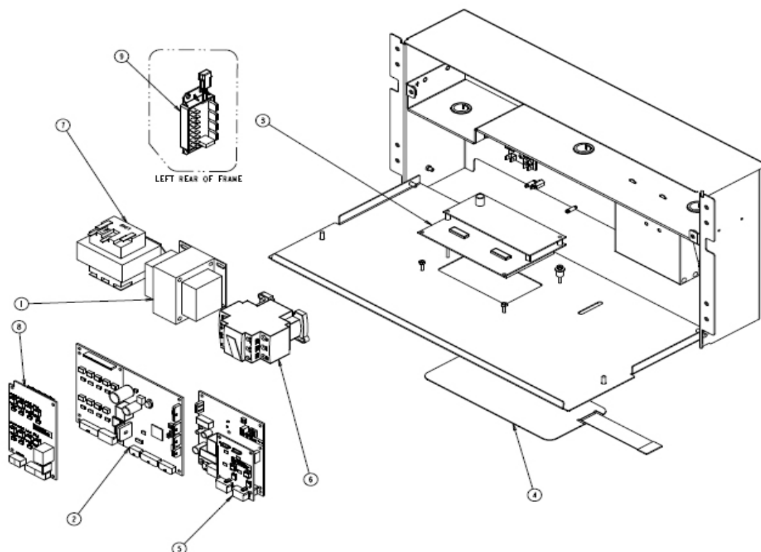
Figure 7. E-Box Assembly
