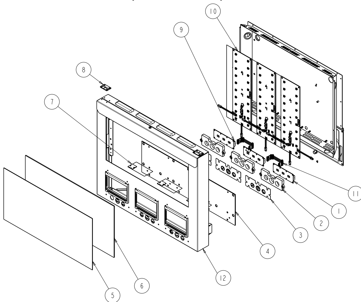
Figure 9. Merchandiser Assembly (Modified Short)
