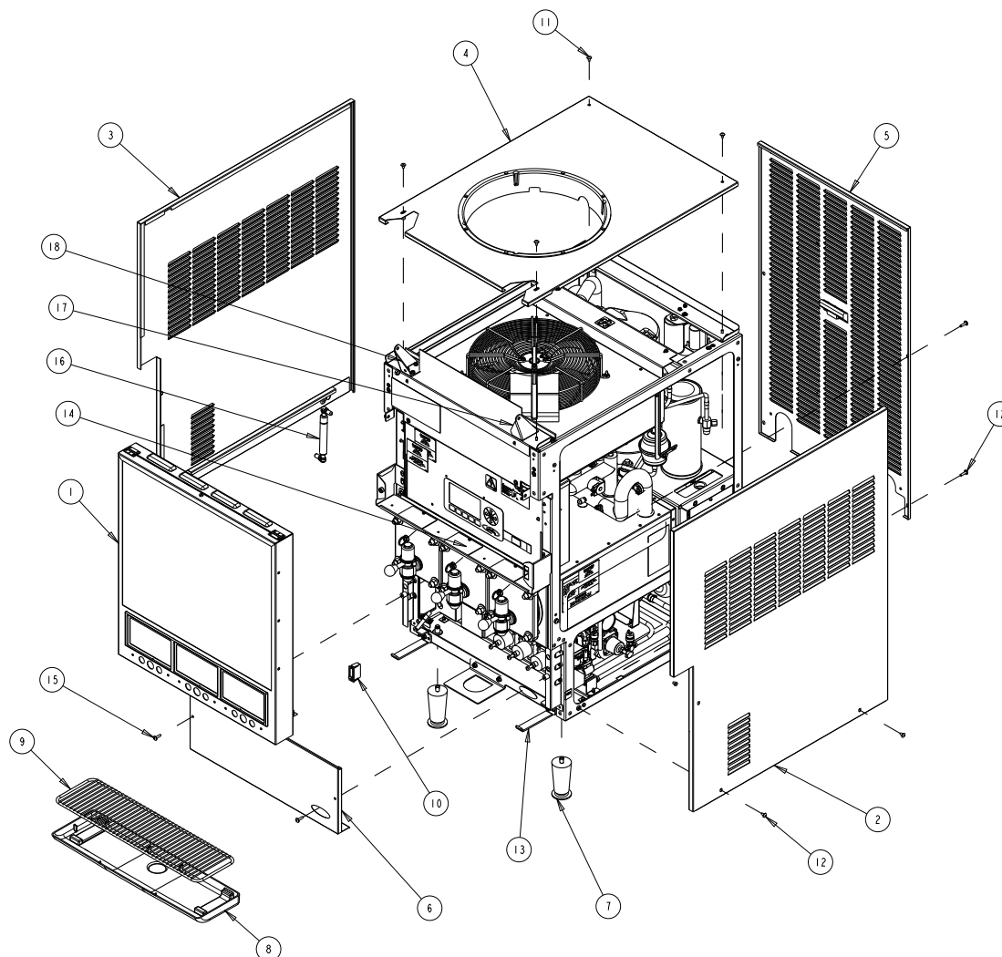
Figure 1. Cladding Assembly
