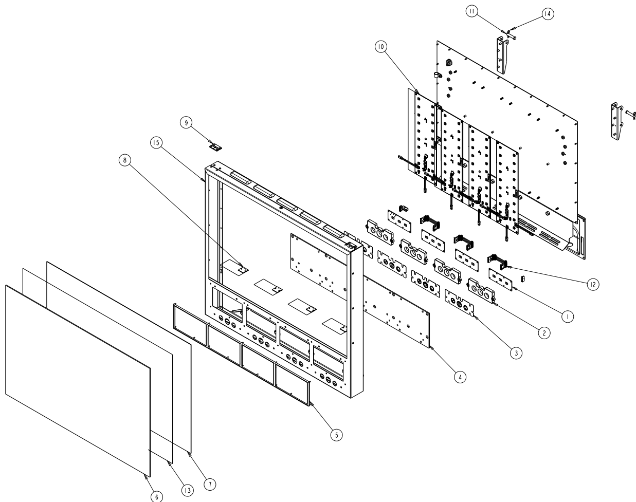
Figure 8. Merchandiser Assembly
