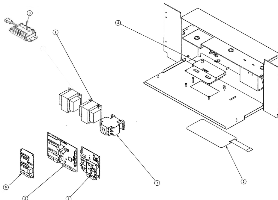
Figure 7. E-Box Assembly
