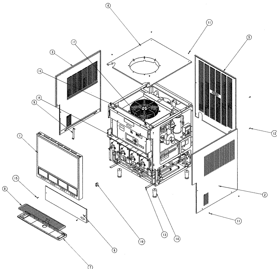
Figure 1. Cladding Assembly
