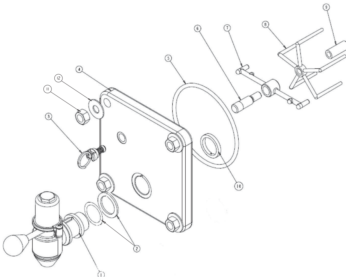
Figure 3. Faceplate Assembly
