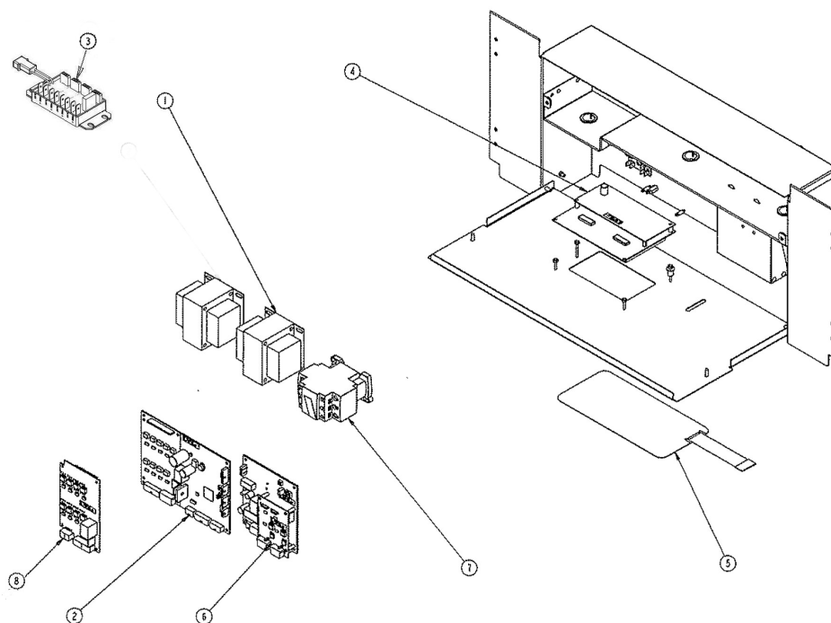
Figure 8. E-Box Assembly
