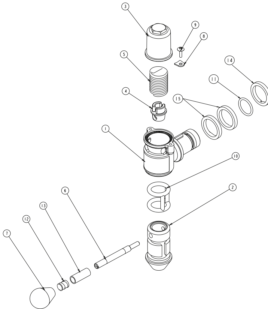
Figure 5. Motorman Valve Assembly
