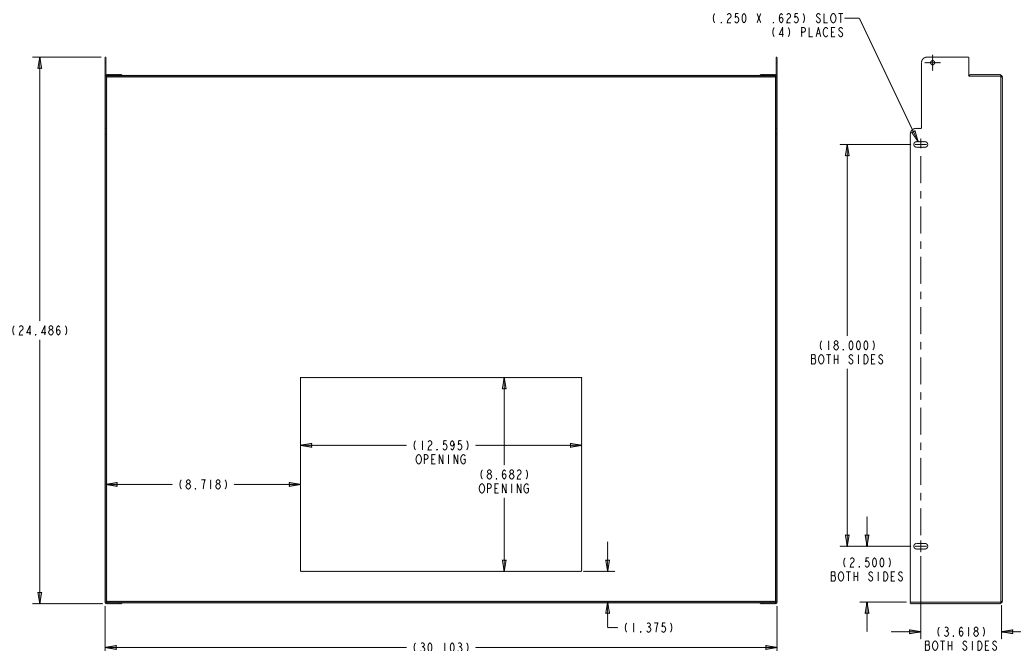
Figure 5. Reference Sheetmetal Cover Opening Dimensions for Mounting Ice Maker.
