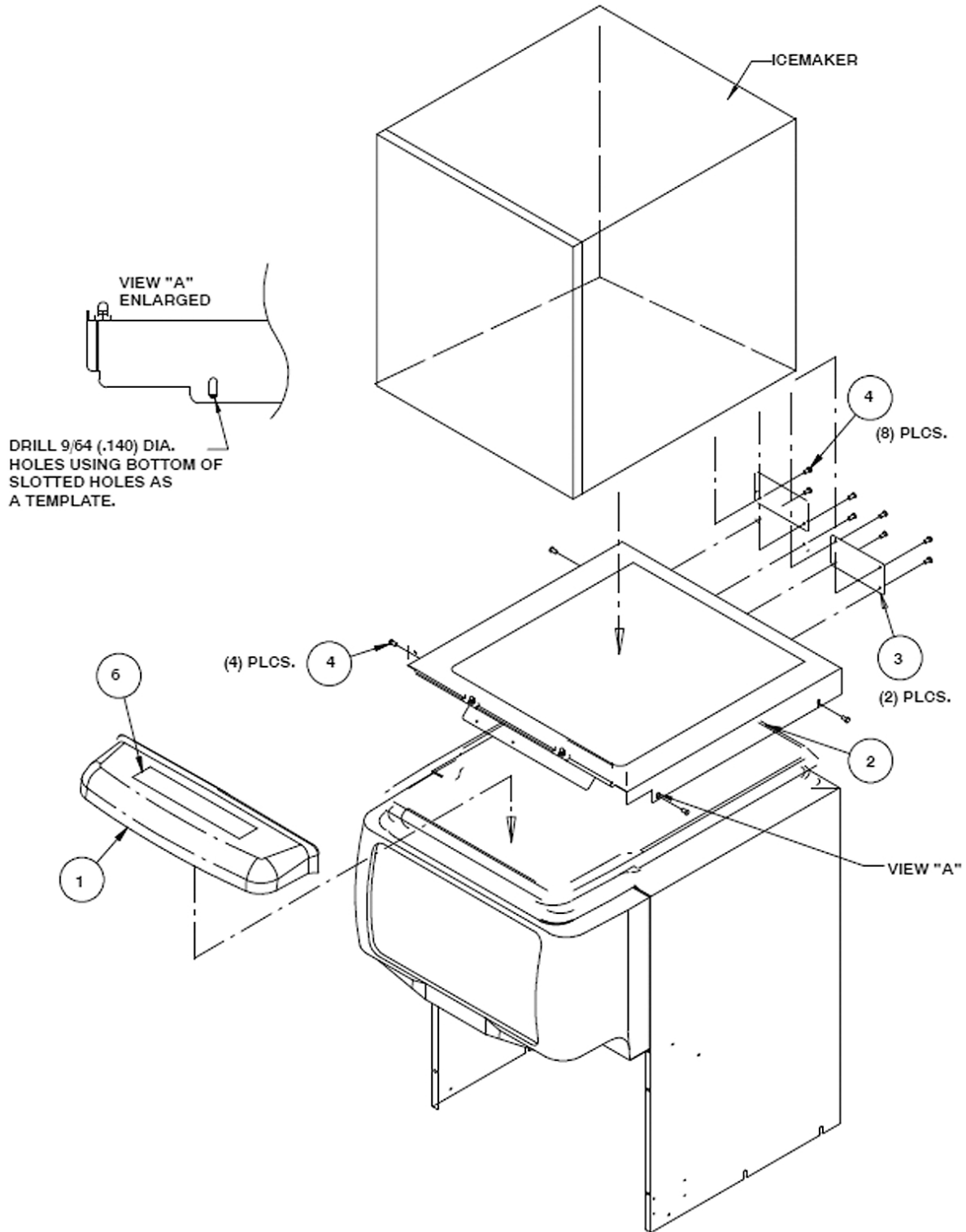
Figure 2. Dispenser Assembly
