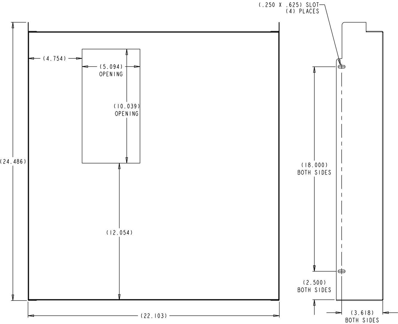
Figure 3. Reference Sheetmetal Cover Opening Dimensions for Mounting Icemaker.
