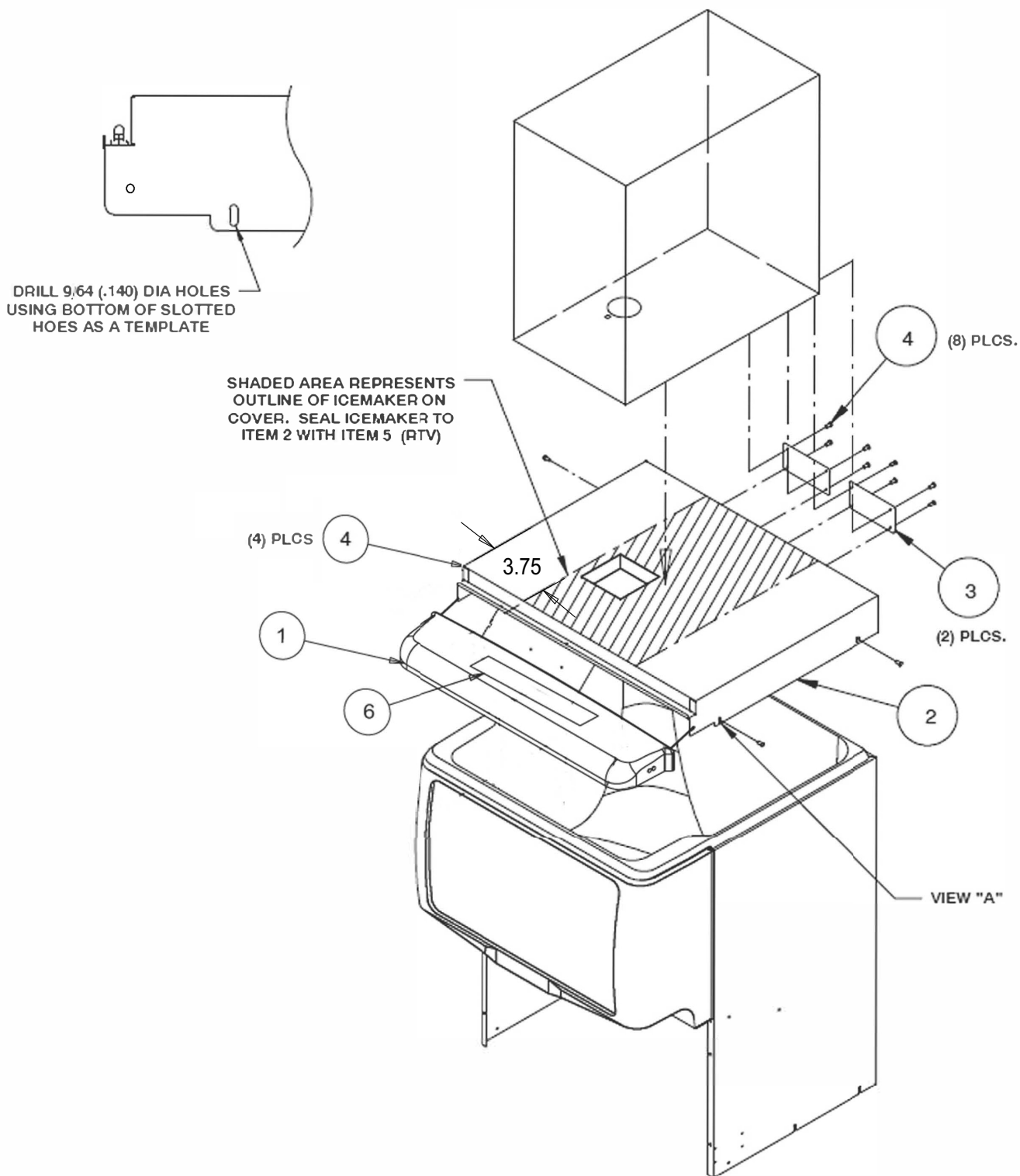
Figure 2. Dispenser Assembly
