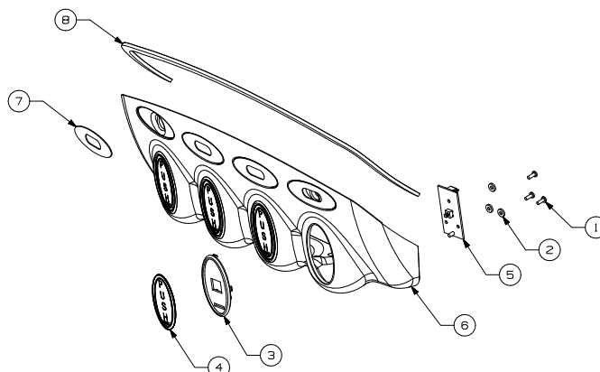
Figure 7. Lower Door Panel Assembly - Push Button - P/N 720508704
