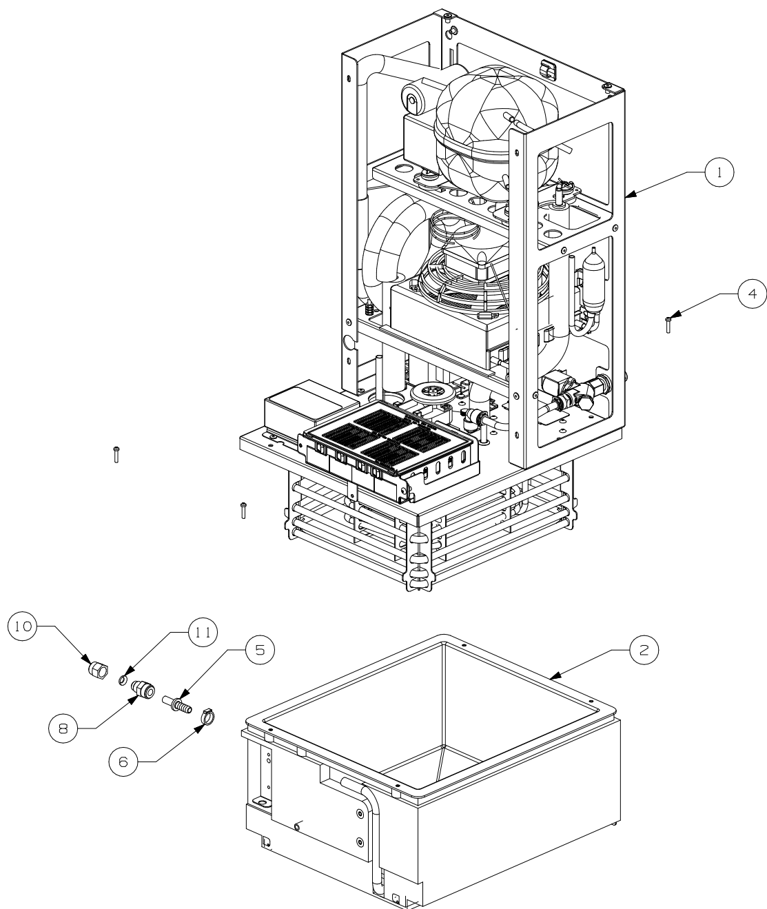
Figure 2. Refrigeration Chassis Assembly, QST NT- P/N 720201914 (115VAC) and P/N 720201913 (230VAC)
