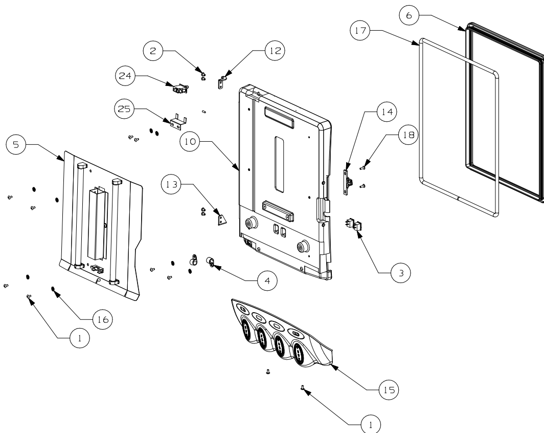
Figure 6. Door Assembly, QST NT - P/N 720500704 PB (115VAC) and P/N 720500705 PC (230VAC)
