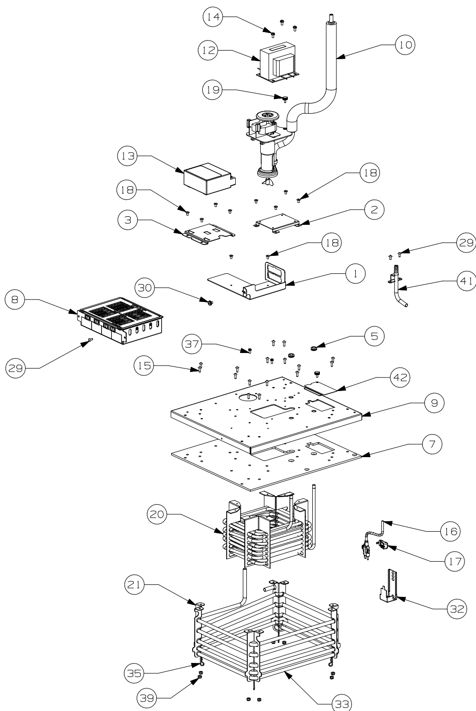
Figure 4. Tank Cover Assembly, QST NT - P/N 720201716 (115VAC) and P/N 720201717 (230VAC)
