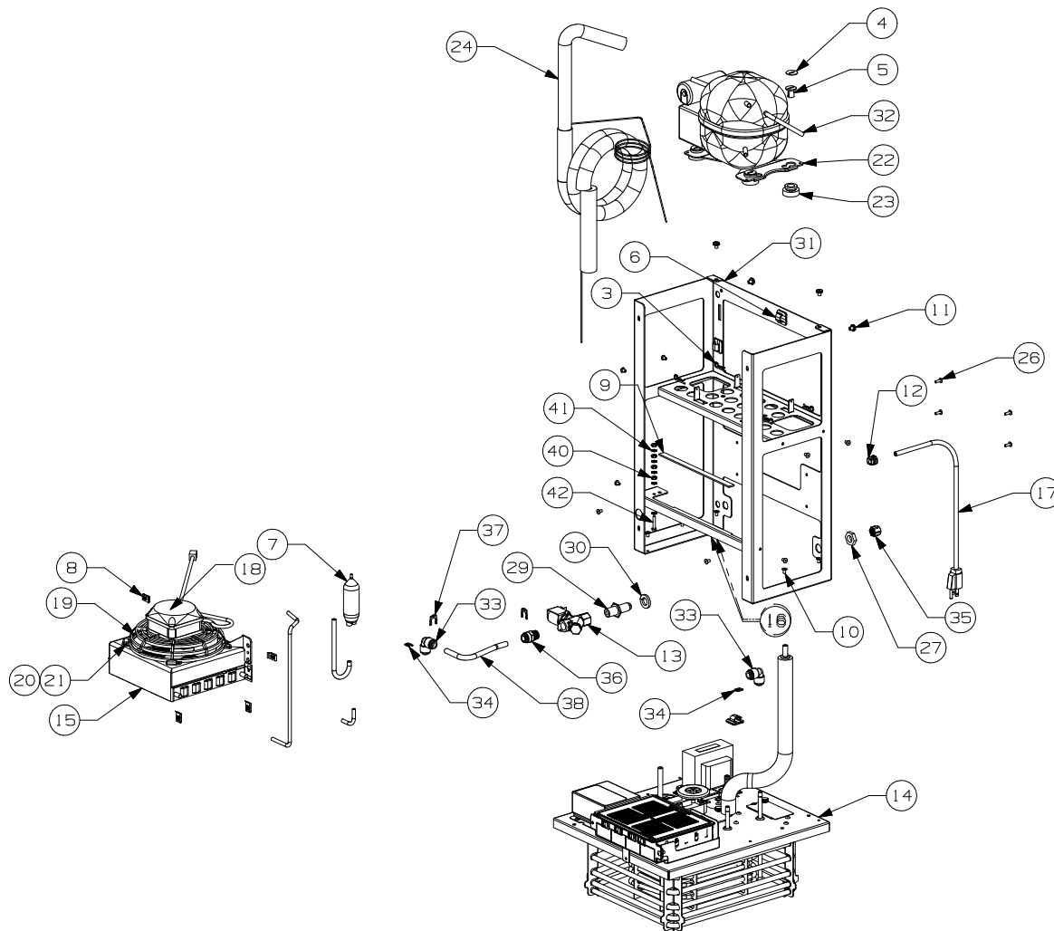
Figure 3. Refrigeration Frame Assembly, QST NT - P/N 720201924 (115VAC) and P/N 720201925 (230VAC)
