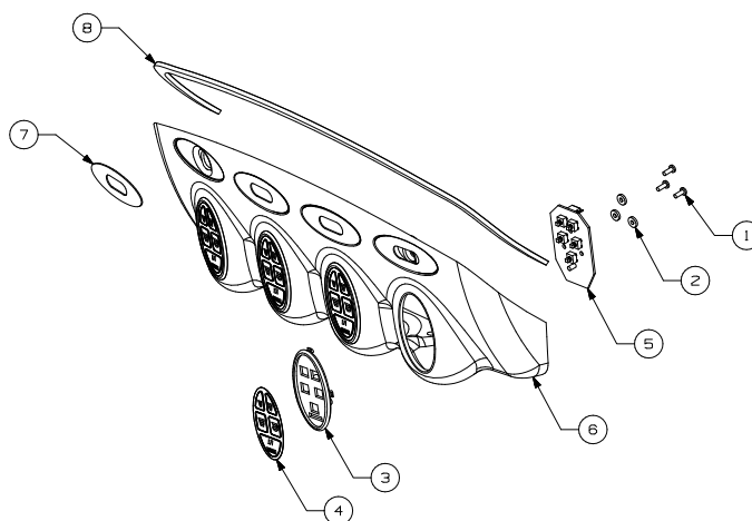
Figure 8. Lower Door Panel Assembly - Portion Control - P/N 720508705
