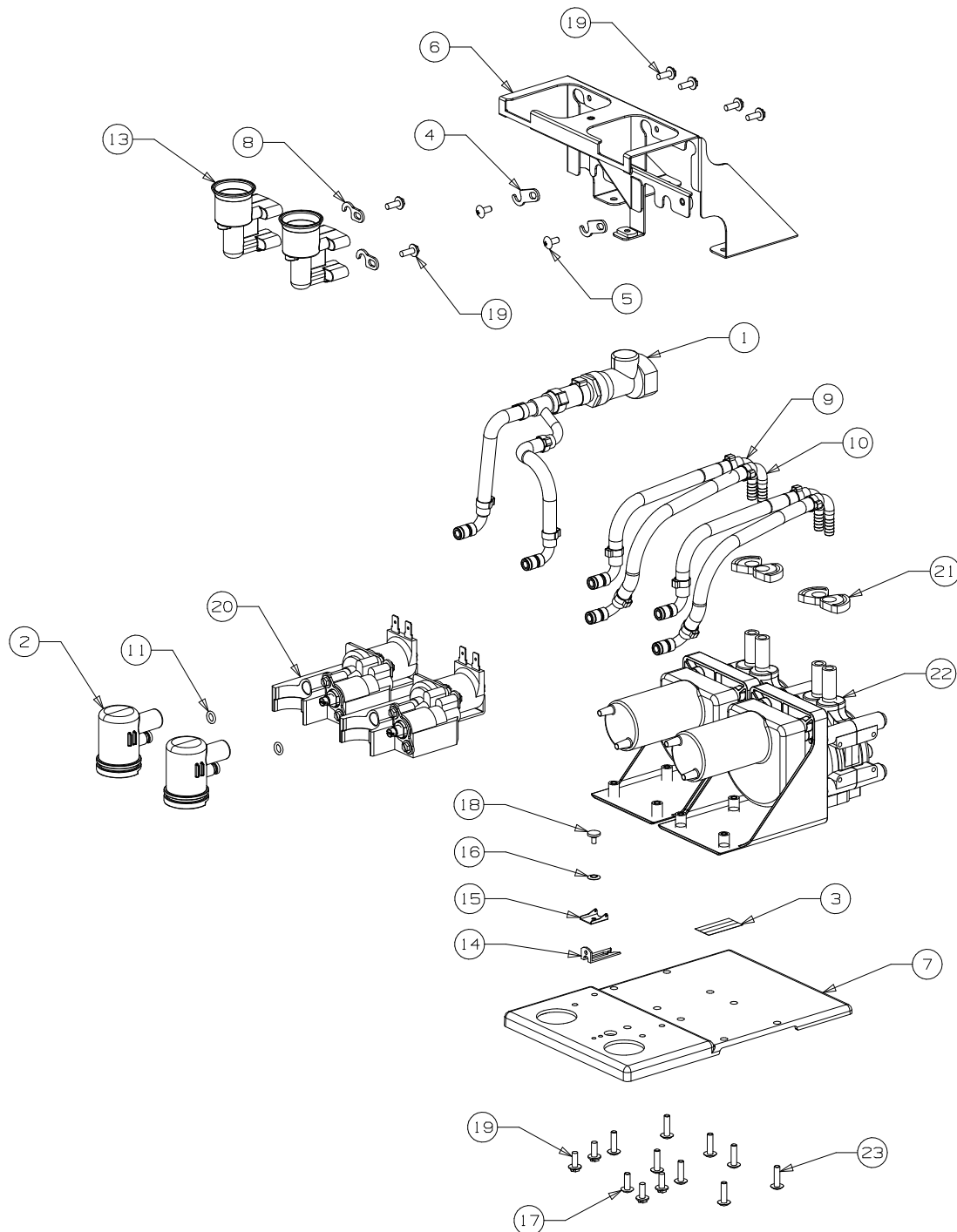
Figure 10. Platform Assembly without Flush/Dispense Option, QST NT - P/N 720401809
