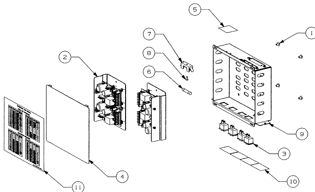
Figure 14. Electrical Box Assembly - P/N 720504304
