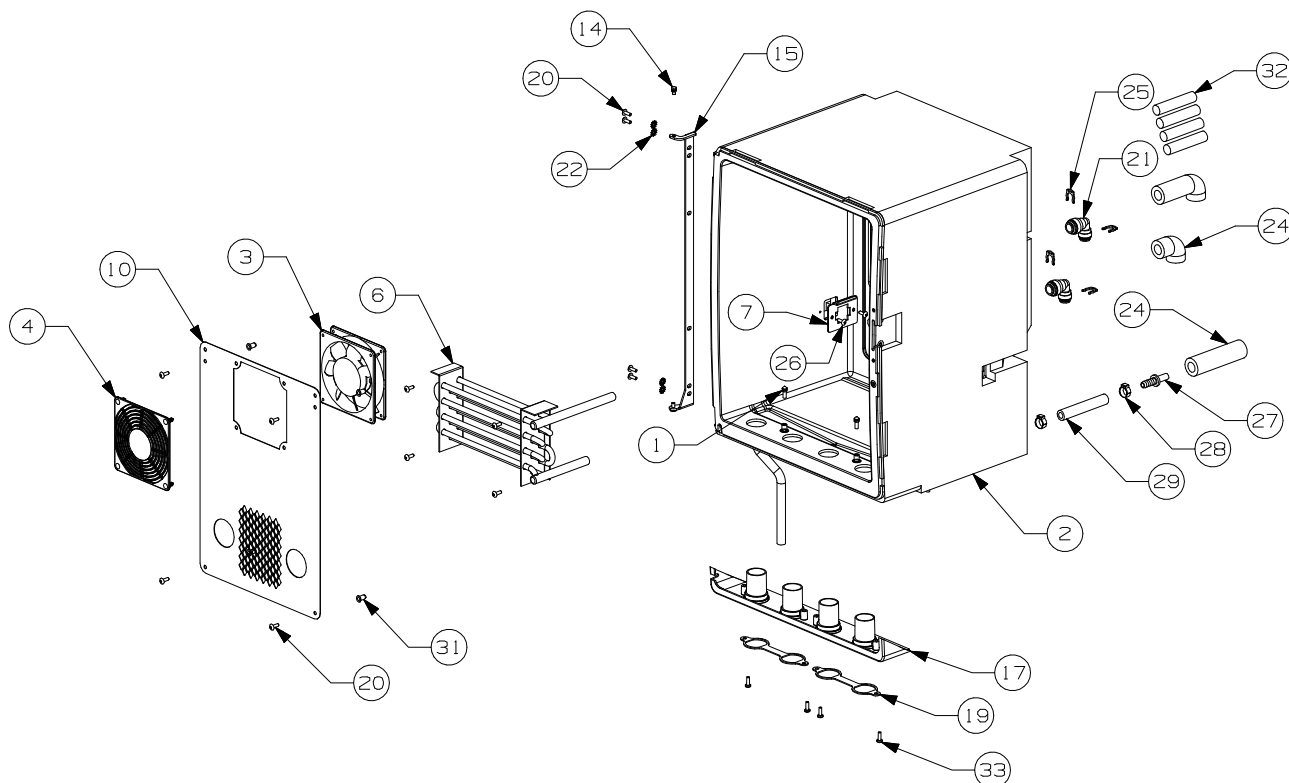
Figure 5. Cabinet Assembly, QST NT - P/N 720505204 (115VAC) and P/N 720505205 (230VAC)
