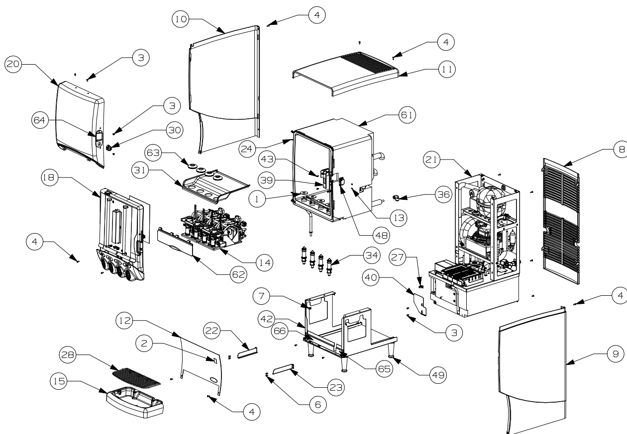
Figure 1. QST NT Final Assembly
