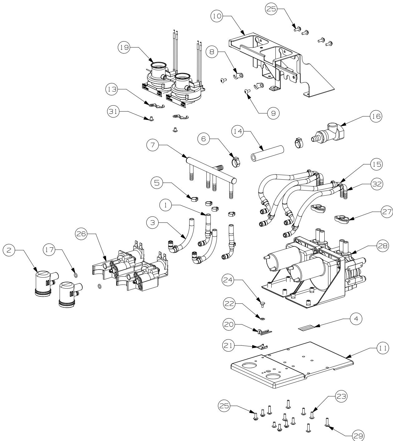
Figure 9. Platform Assembly with Flush/Dispense Option, QST NT - P/N 720401801
