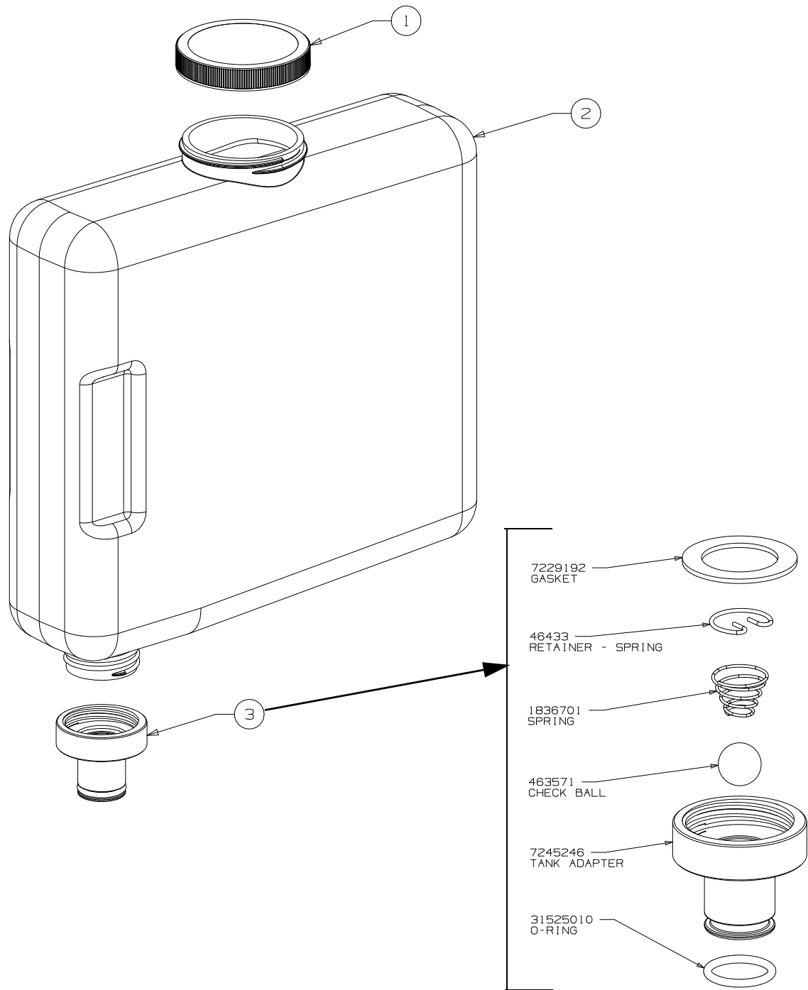
Figure 15. Generic Bottle Assembly - P/N 720500066
