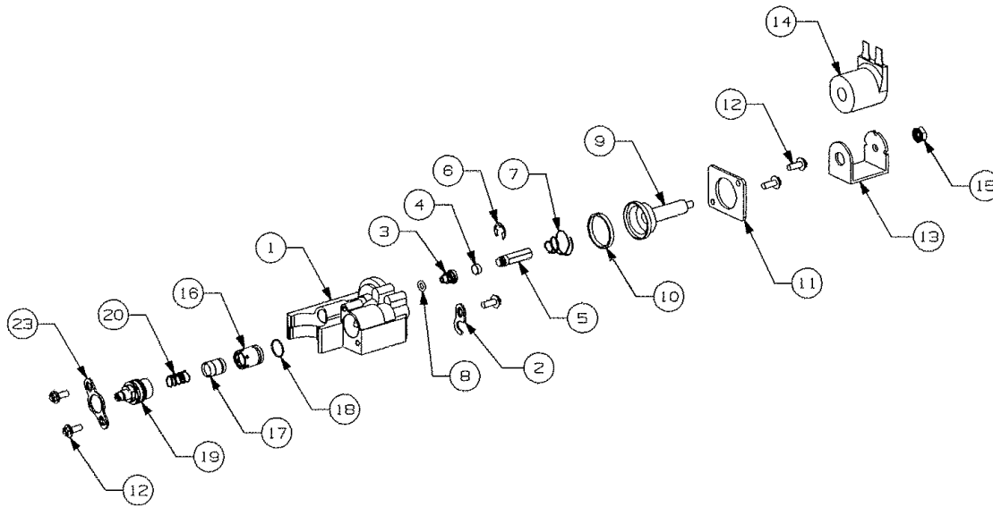
Figure 13. Valve Block Assembly - P/N 45508200
