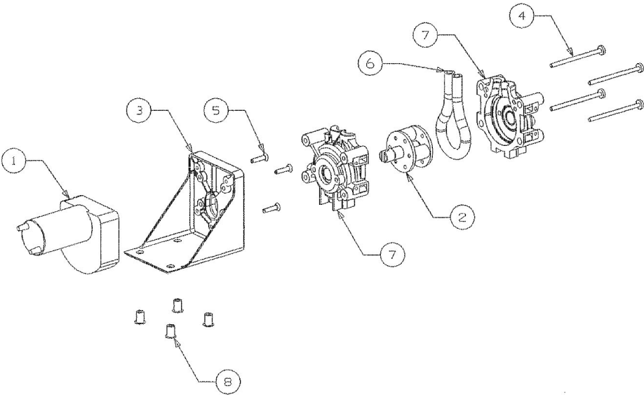
Figure 11. Pump Assembly - P/N 45185
