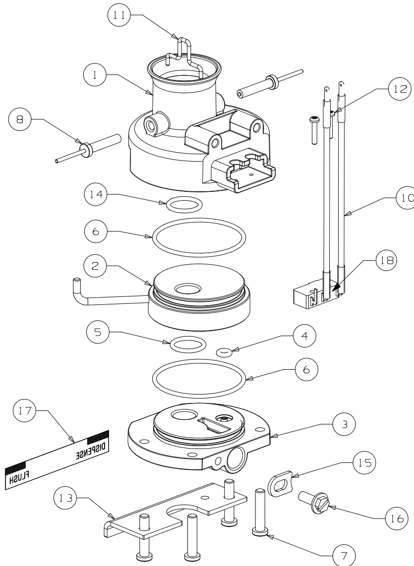
Figure 12. Bottle Adapter Assembly - P/N 45026
