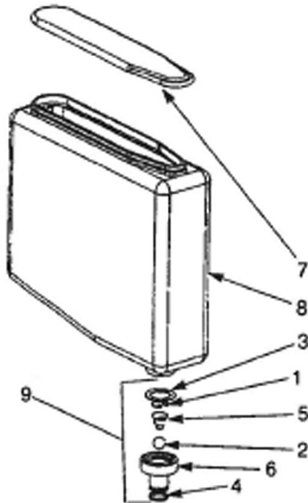
Figure 14.. Tank Assembly
