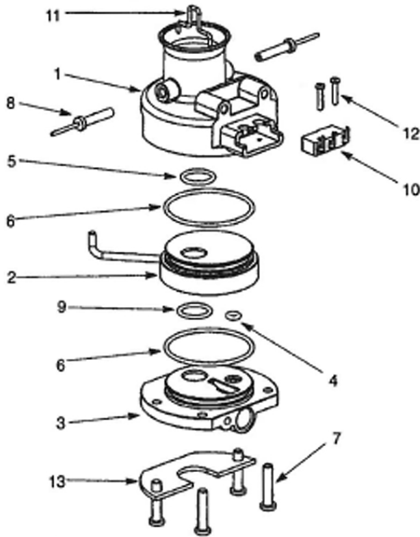
Figure 6. Bottle Adapter Assembly
