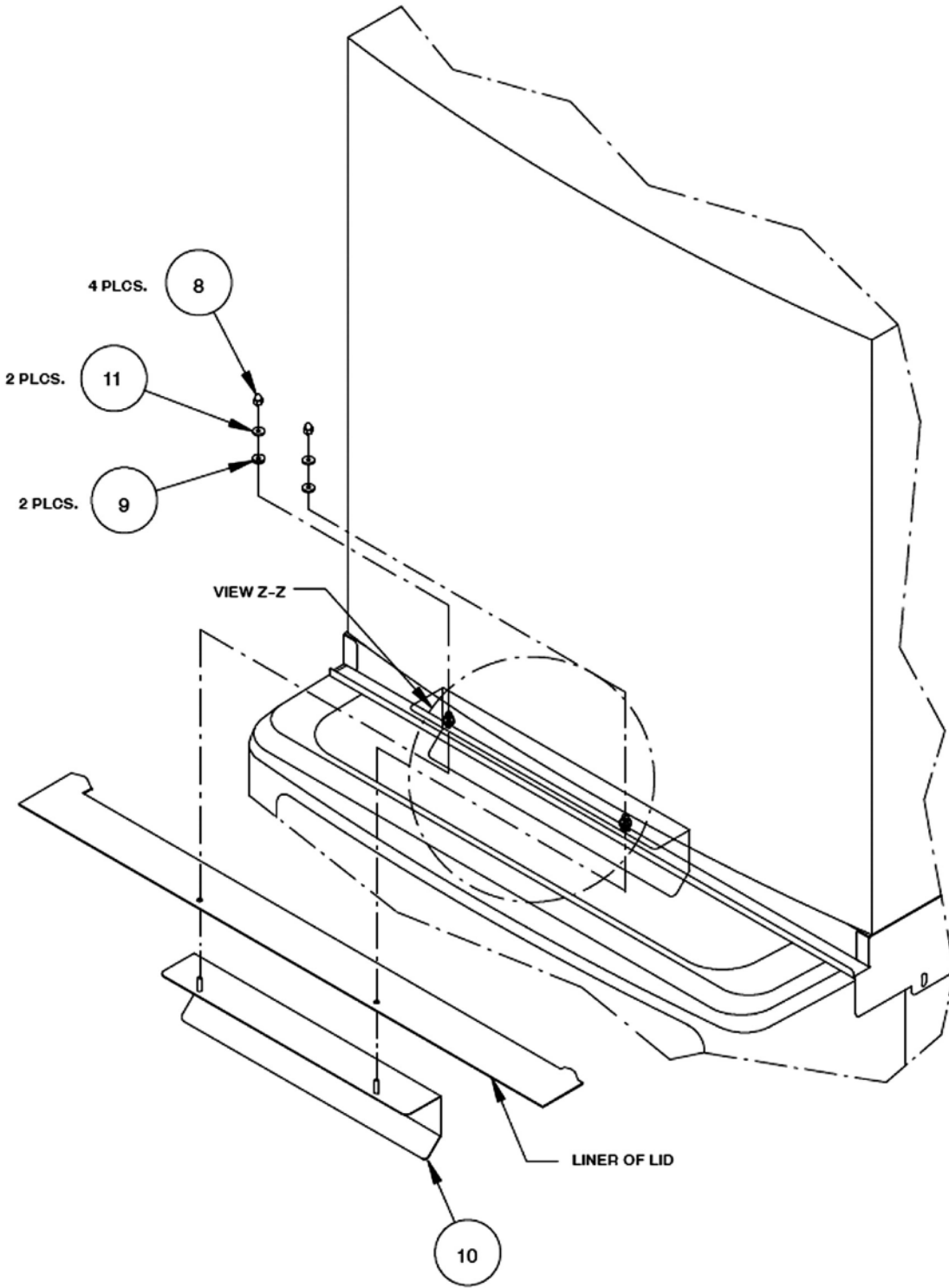
Figure 2. ED150 Kit
