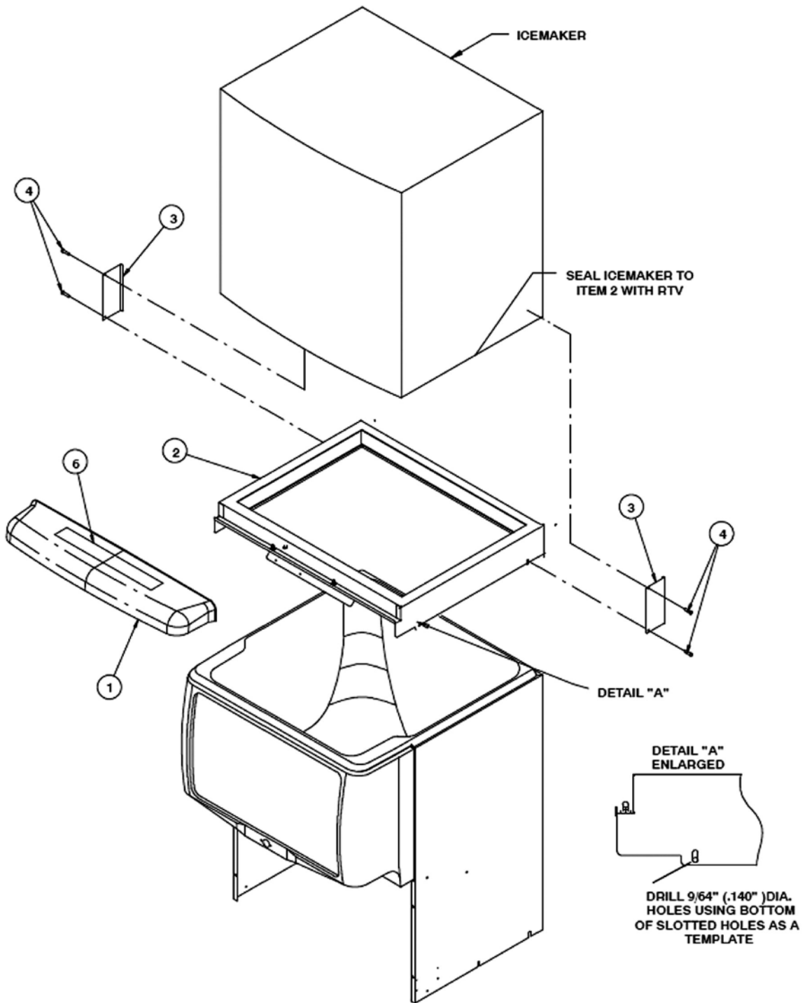
Figure 1. Dispenser Assembly
