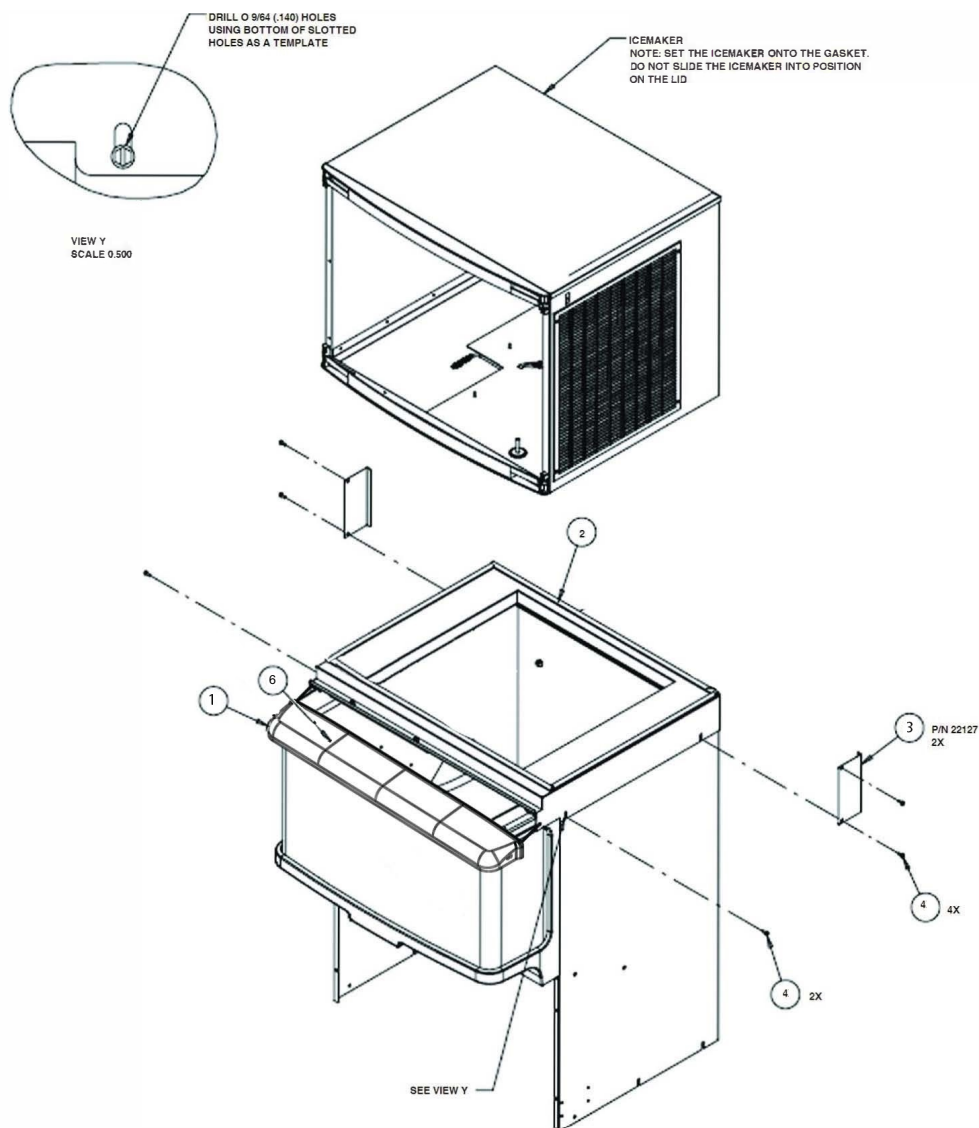
Figure 2. Dispenser Assembly
