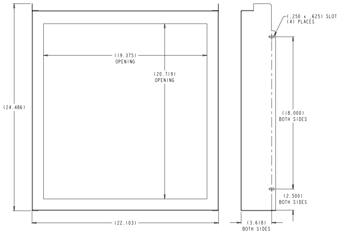
Figure 5. Reference Sheetmetal Cover Opening Dimensions for Mounting Ice Maker.
