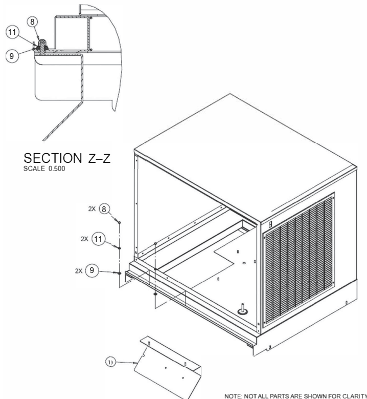
Figure 1 Parts
