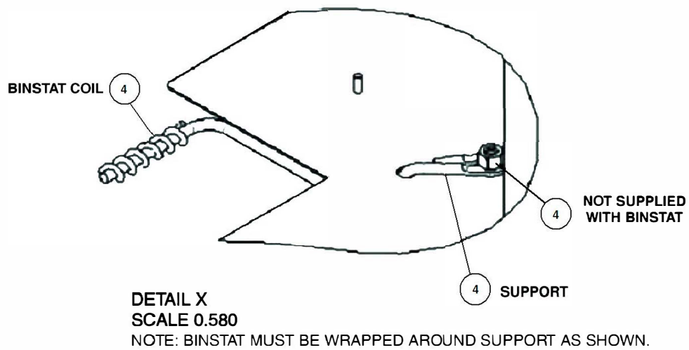
Figure 4. Detail X
