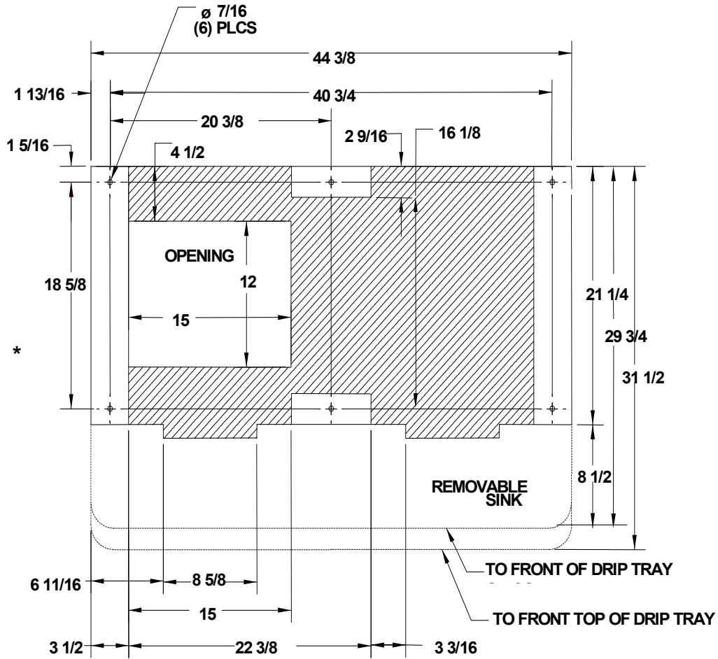
Figure 2. Mounting Template
