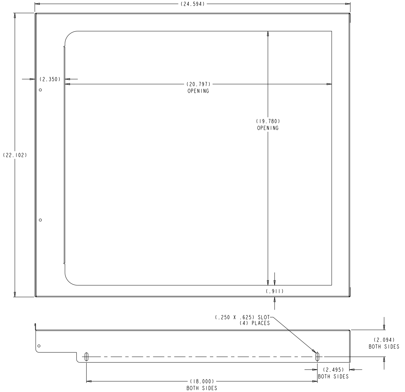
Figure 3. Reference Sheetmetal Cover Opening Dimensions for Mounting Ice Maker
