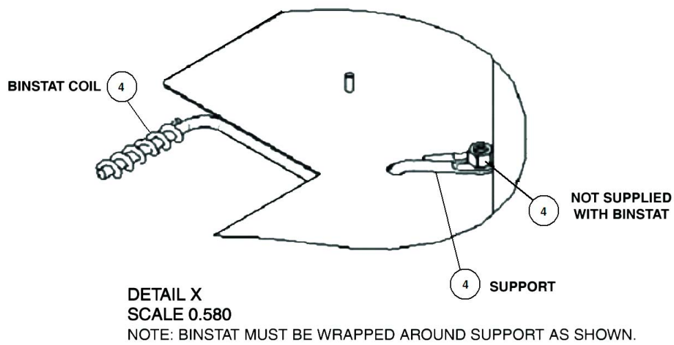
Figure 4. Detail X
