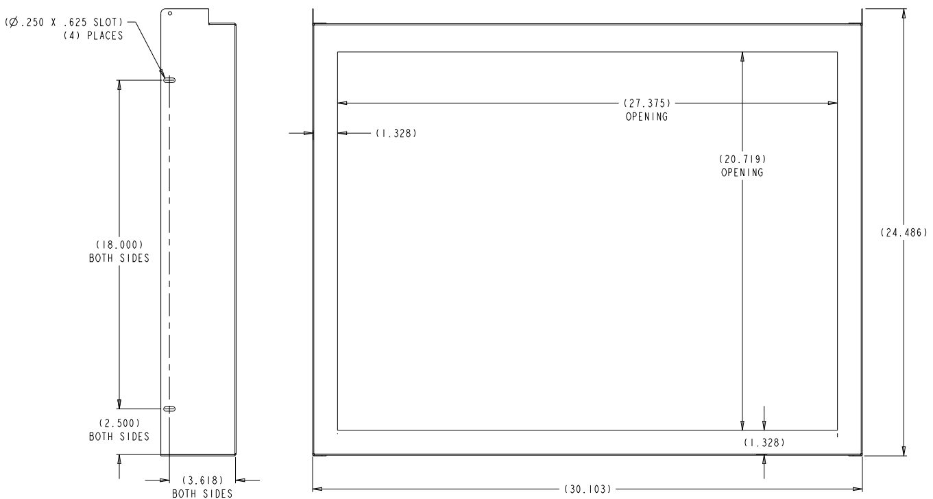
Figure 5. Reference Sheetmetal Cover Opening Dimensions for Mounting Icemaker.
