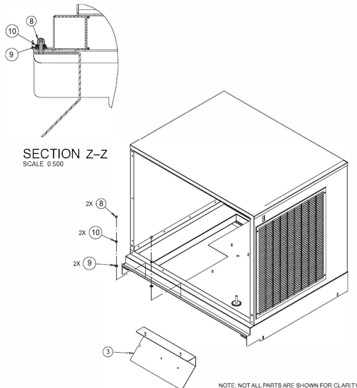
Figure 1 Parts
