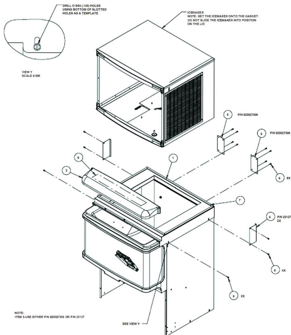
Figure 2. Dispenser Assembly
