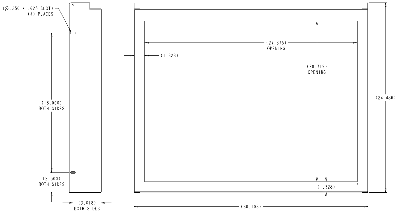
Figure 4. Reference Sheetmetal Cover Opening Dimensions for Mounting Icemaker.
