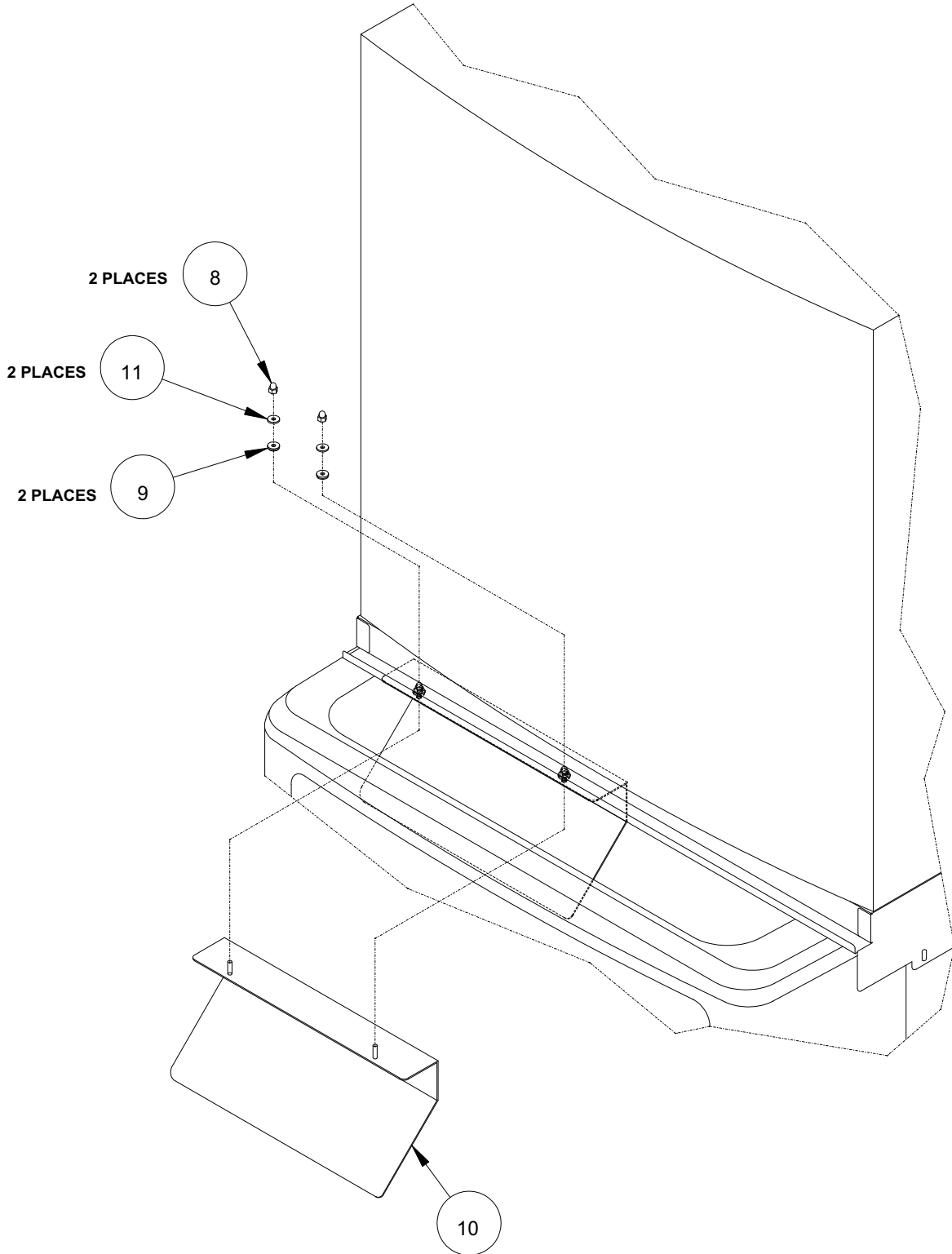
Figure 2. ED2XX KIT
