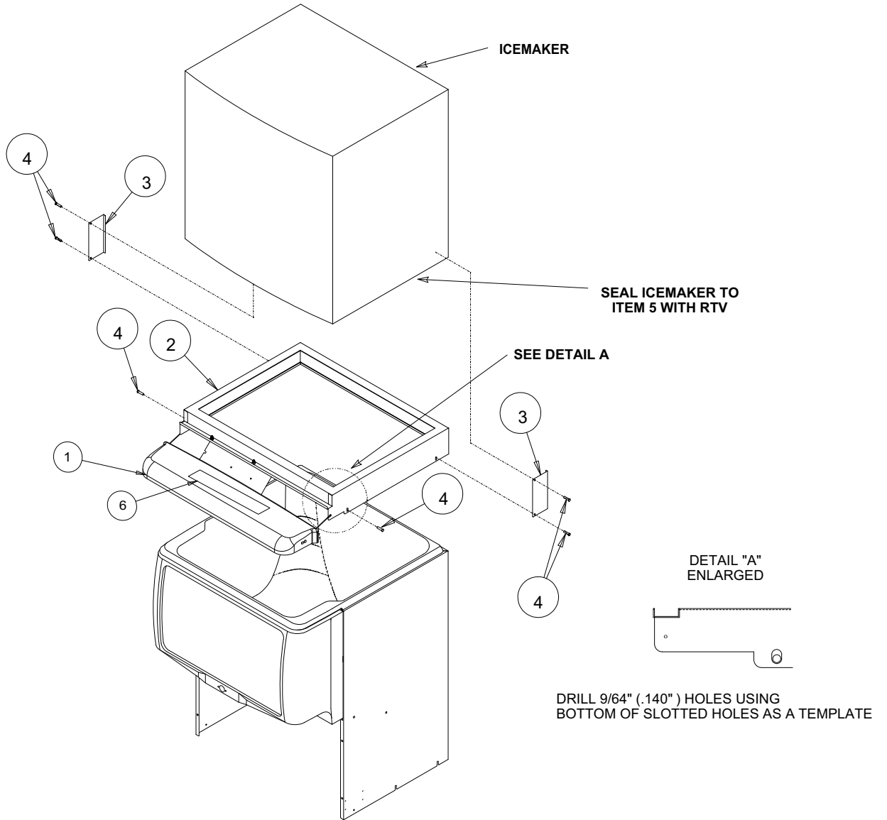
Figure 1. Dispenser Assembly
