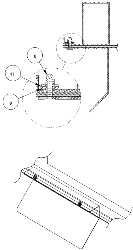
Figure 3. ED2XX KIT
