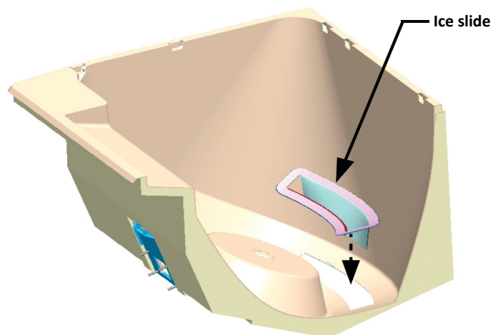
Figure 2. Ice Slide Assembly
