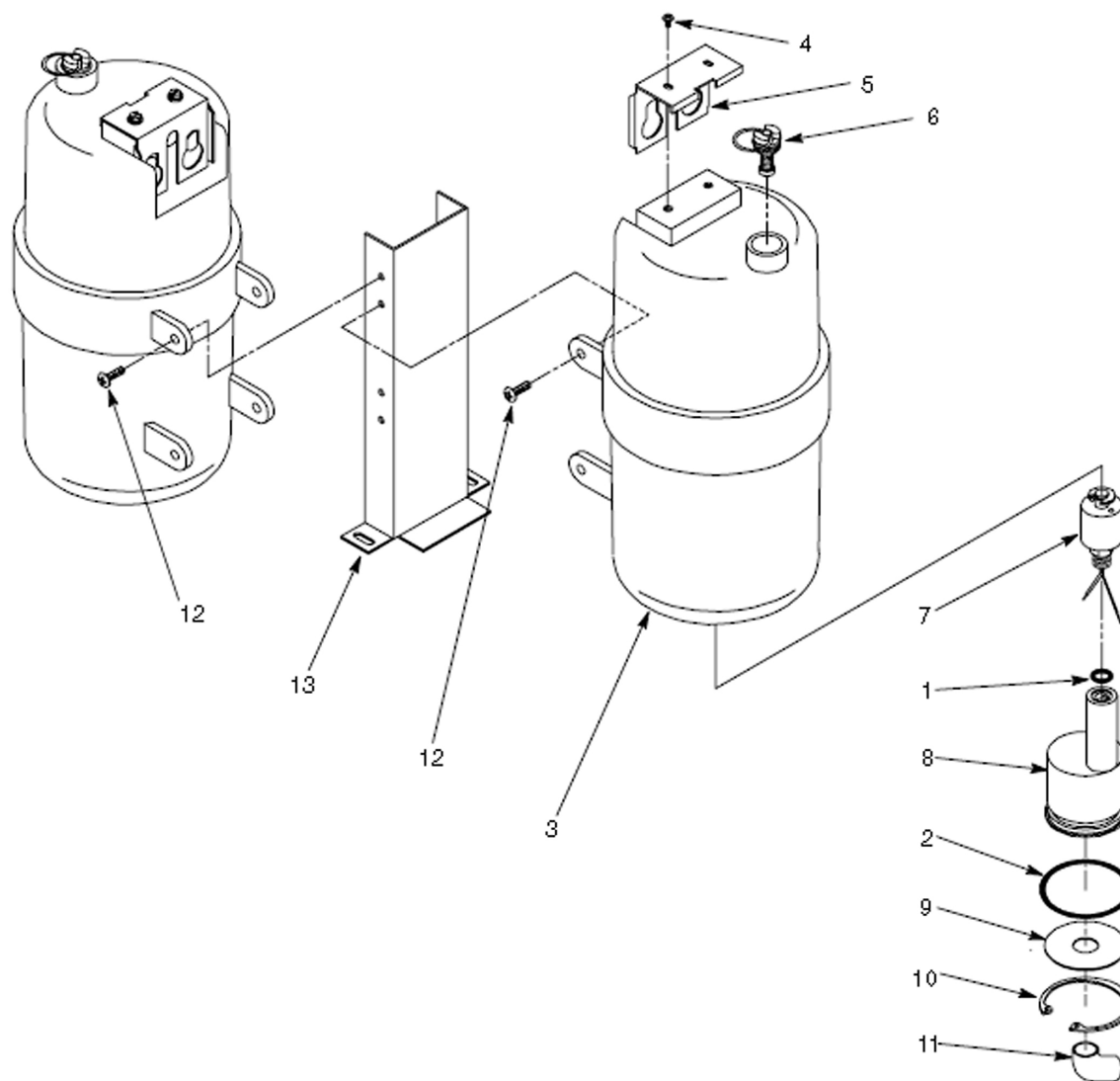
Figure 15. Blender Components
