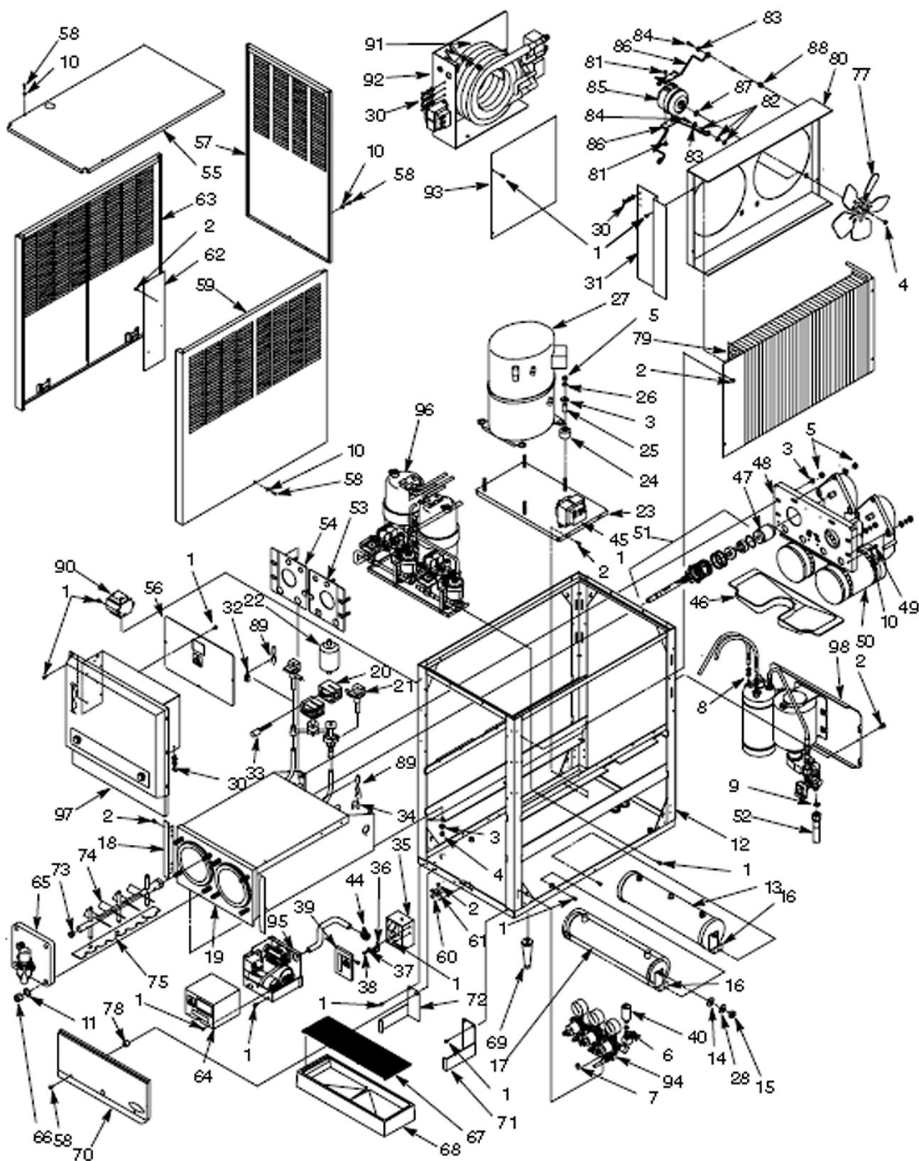
Figure 1. Overcounter FCB Post-Mix Dispenser
