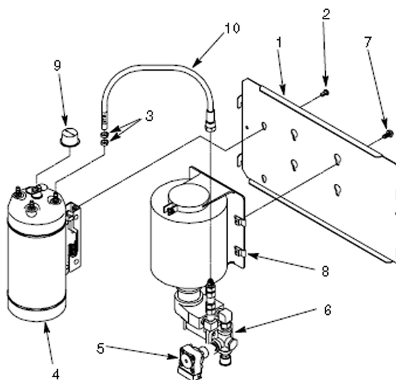
Figure 19. Carbonator Components
