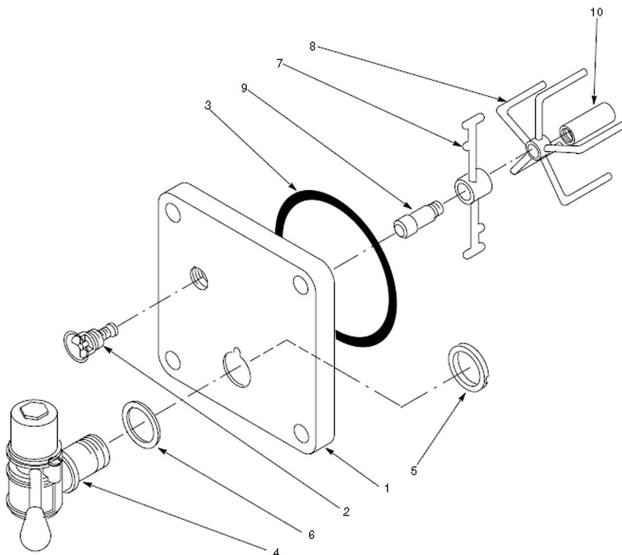
Figure 17. Faceplate Assembly
