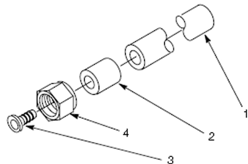
Figure 6. Tube Assembly
