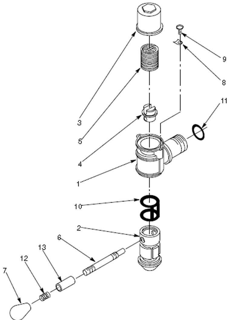
Figure 18. Dispensing Valve Assembly
