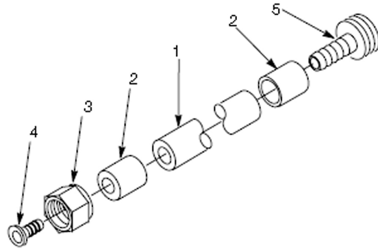
Figure 12. Tubing Assembly (Regulator to Blender)
