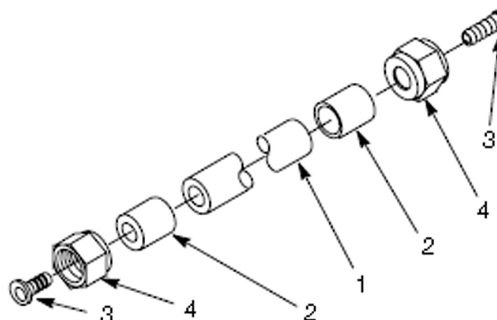
Figure 20. Tubing Assembly
