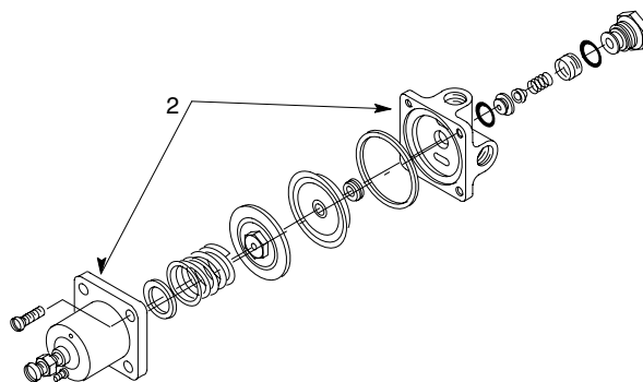
FIGURE 14. CO 2 REGULATOR COMPONENTS
