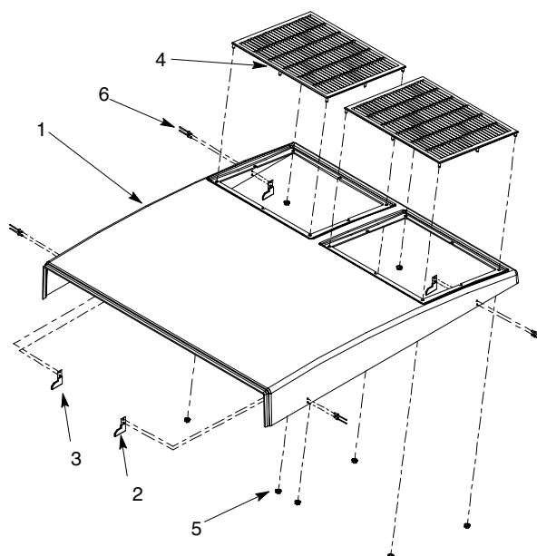
FIGURE 32. TOP COVER ASSEMBLY
