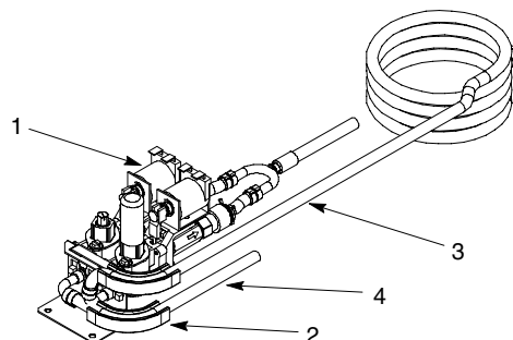
FIGURE 26. BRIX LINE 4 COMPONENTS
