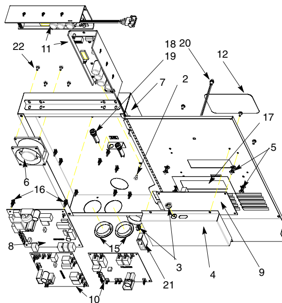
FIGURE 31. 2FL CONTROL BOX ASSEMBLY
