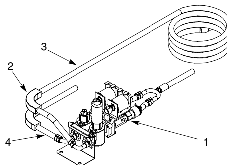
FIGURE 23. BRIX LINE 1 COMPONENTS
