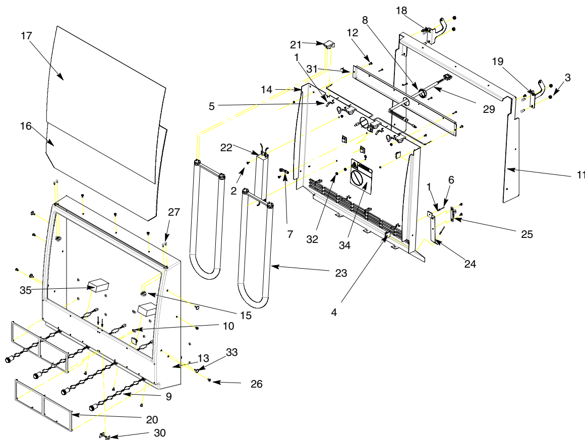
FIGURE 33. MERCHANDISER ASSEMBLY
