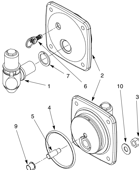
FIGURE 9. FREEZE DOOR ASSEMBLY
