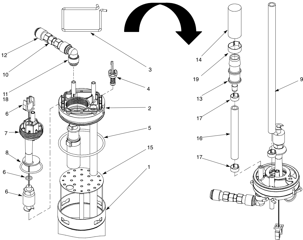
FIGURE 2. BLENDONATOR ASSEMBLY
