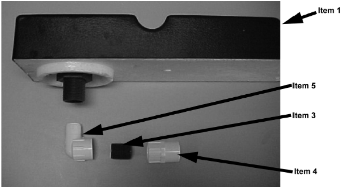
Figure 2. Fittings included in kit
