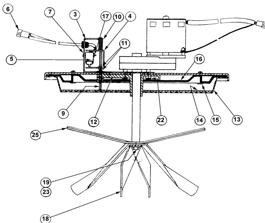
SIDE VIEW ICE LEVEL CONTROL ASSEMBLY IMD 300-30 AND 600-30
