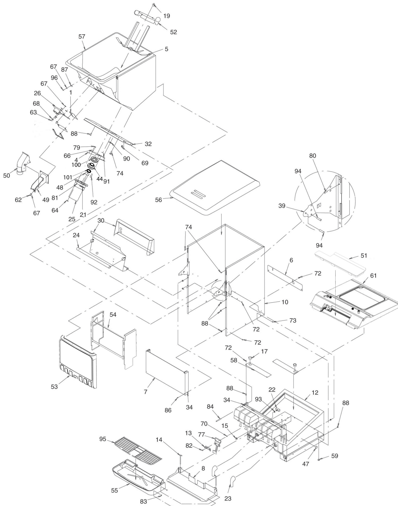
Figure 1. Cabinet Section Exploded View
