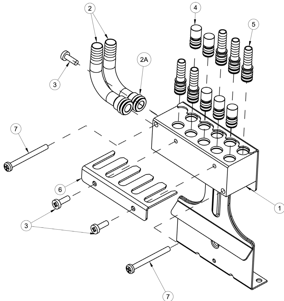
Figure 9. Water Manifold Assembly
