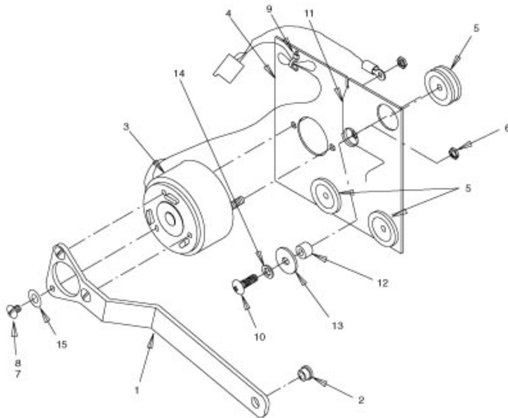
Figure 5. Solenoid Assembly
