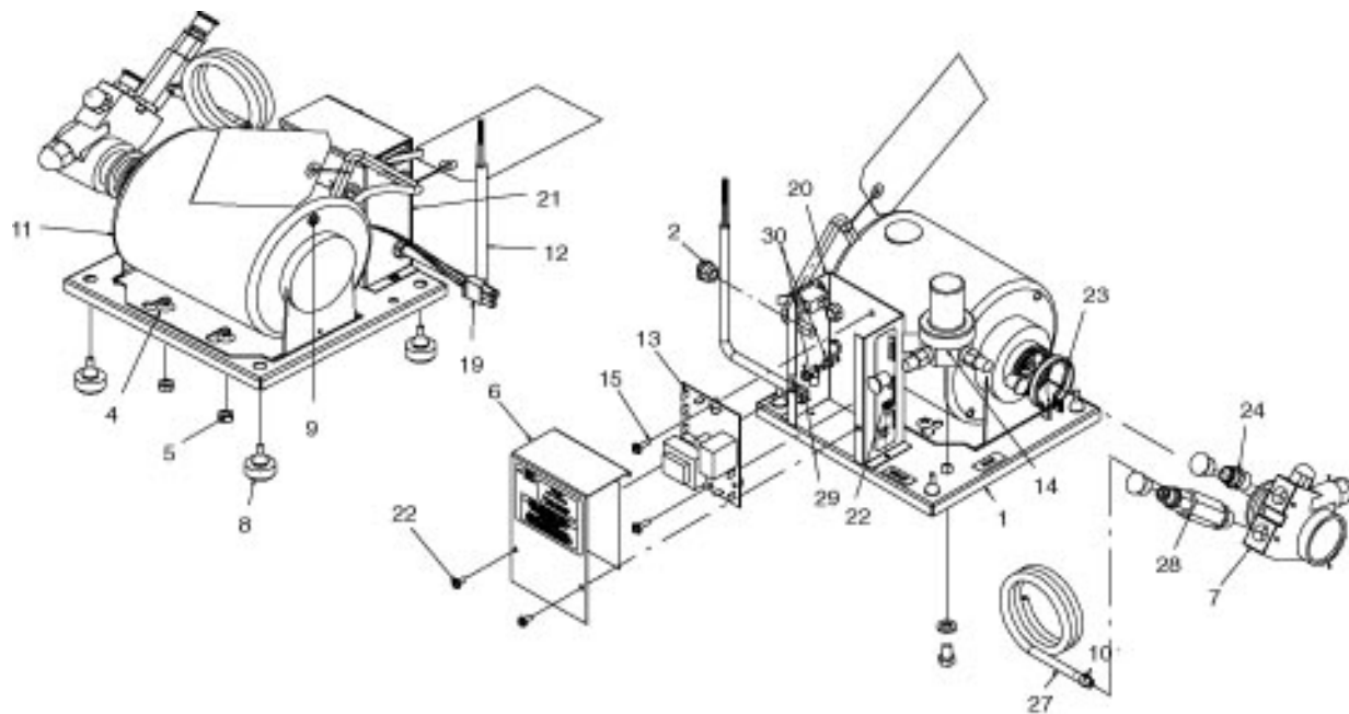
Figure 8. Pump And Motor Assembly
