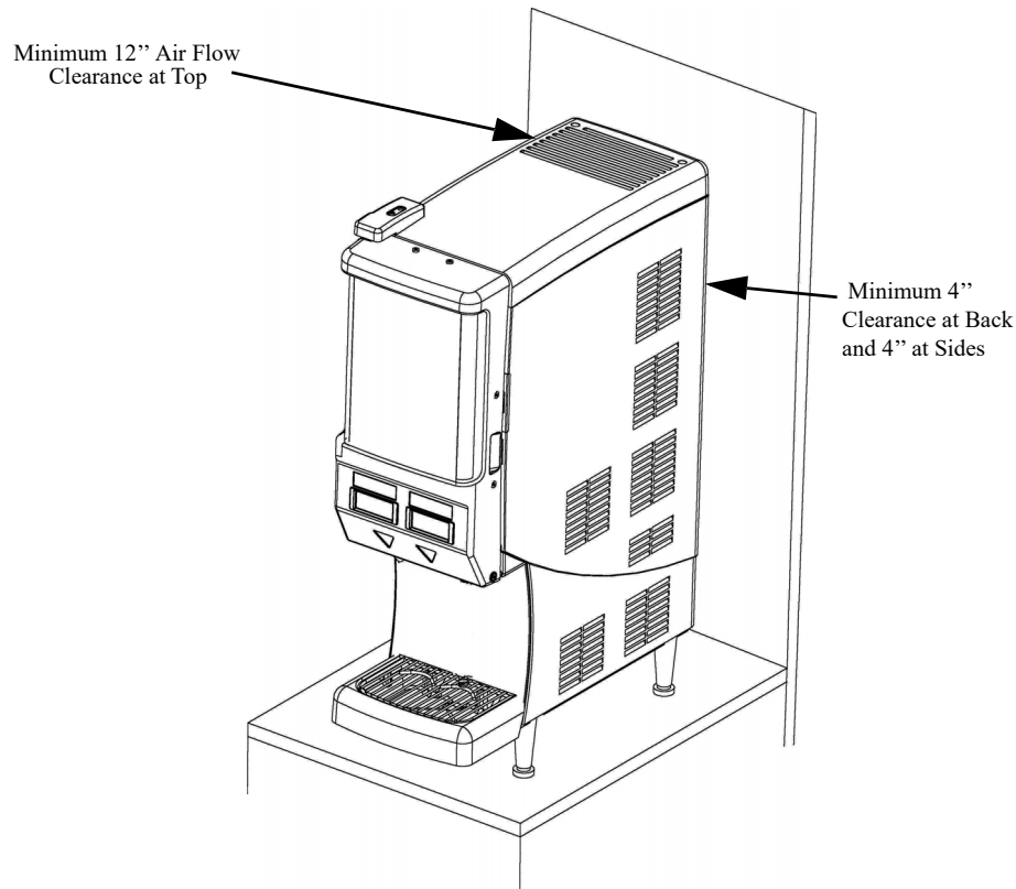
Figure 5. Minimum Clearances
