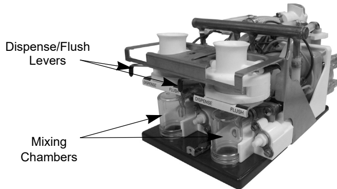
Figure 8. Dispense/Flush Levers
