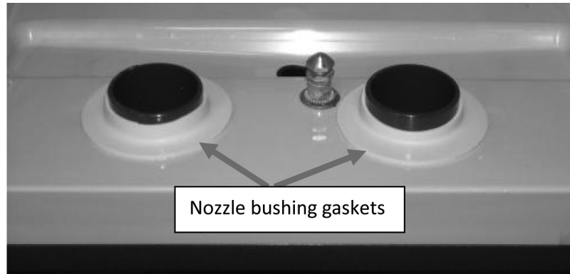
Figure 16. Nozzle bushing gaskets - proper installation
