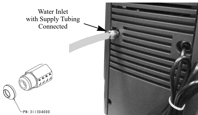
Figure 10. Water Supply Connection on Rear of Unit
