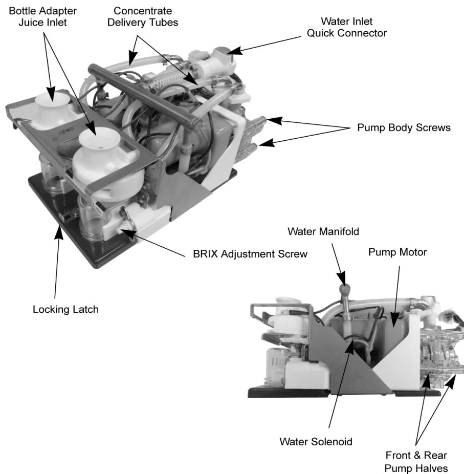
Figure 13. Interior Details
