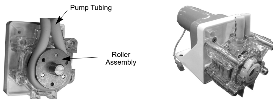
Figure 15. Pump Assembly
