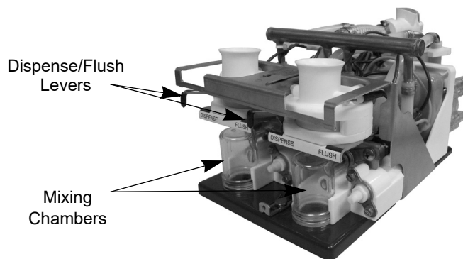
Figure 6. Platform Assembly with Dispense/Flush Levers
